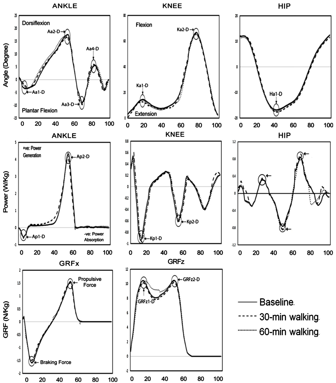
Fig. 4. Dominant side kinematic/kinetic data along a gait cycle with the prescribed insoles (averaged across all subjects).
