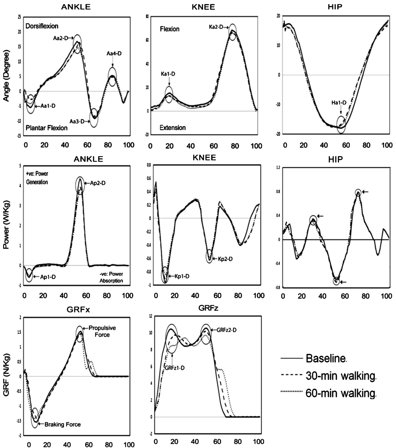
Fig. 3. Dominant side kinematic/kinetic data along a gait cycle without the prescribed insoles (averaged across all subjects).
